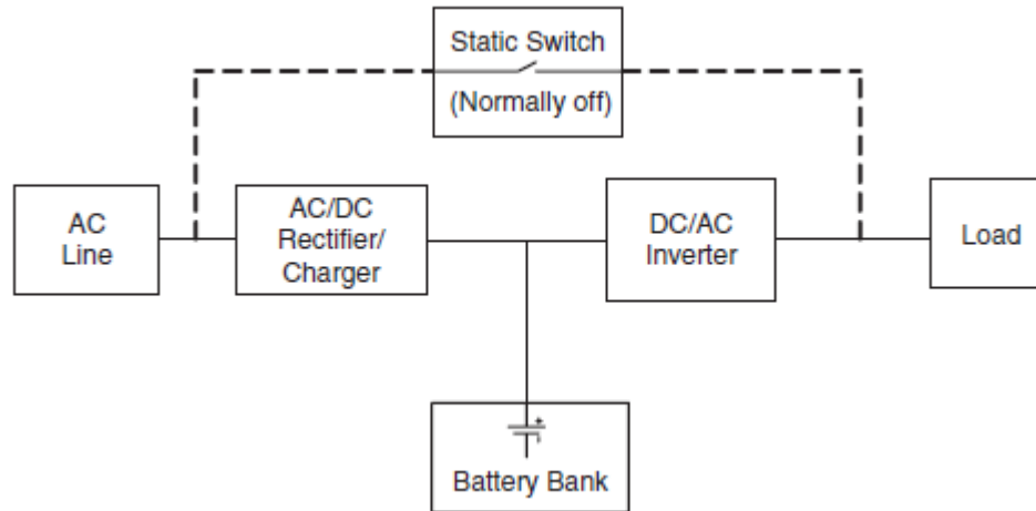
Figure 2: Representing the Online UPS system [Mdpi].
