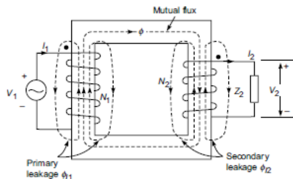
Figure 1: Representing the Real Transformer [EEE Guide].
