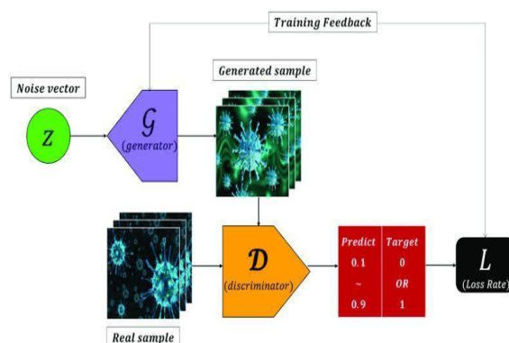
Fig4:GenerativeAdversarialNetwork
