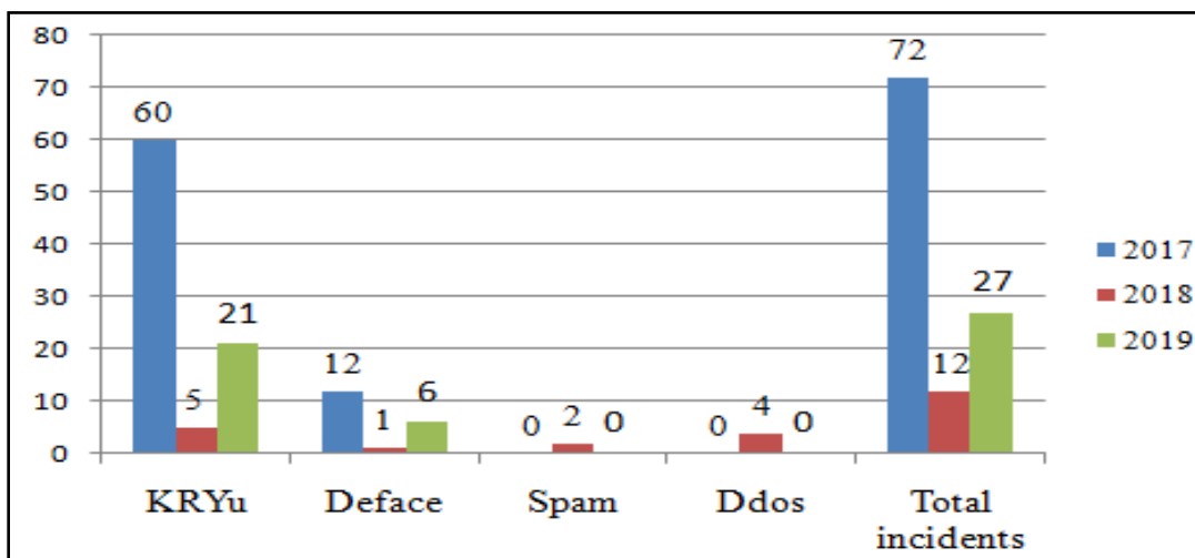
Diagram 3. Dynamics of organized threats to the public sector in 2017-2019
