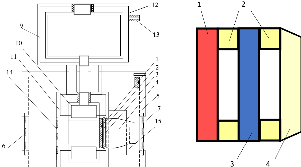
Fig.1, b. Gas discharge cell with n\text{-Si} photodetector and GaAs damping electrode. 1 - n\text{-Si} photodetector; 2 - mica plates with holes in the center; 3 - GaAs; 4 - fiber optic washer with \text{SnO}_2 .
