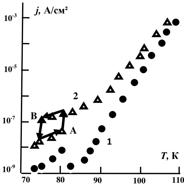
Fig. 2, a. Temperature dependences of the dark (curve 1 - black circles) and photocurrents (curve 2 - light triangles) in a semiconductor photographic ionization camera with a p\text{-Si} \langle Pt \rangle photodetector.
