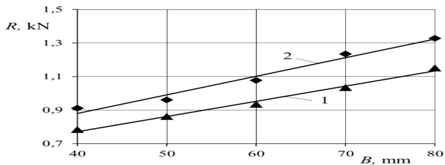
Picture 4. Graph of change of soil compaction rate ( \Phi < 50 ) depending on the width of the working body (V)
